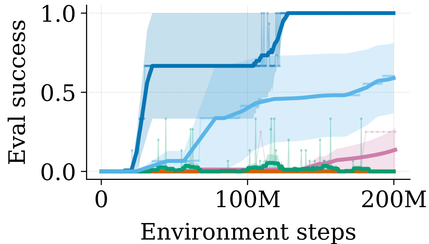
Creative 4 Task 1 · eval (roll. mean w=21 )
