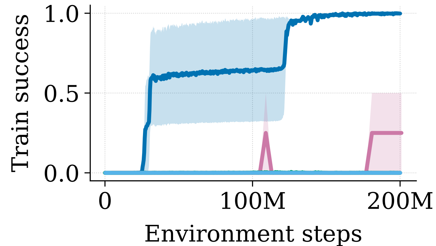
Creative 4 Task 1 · train
